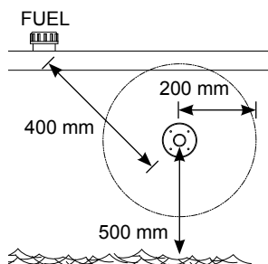
Safety distances
