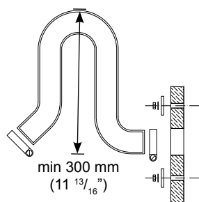
Goose neck
